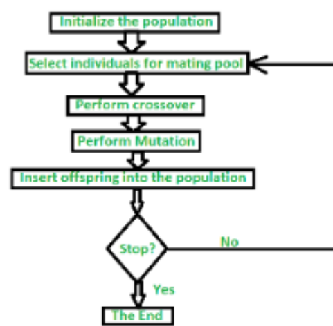
Fig. 3.9 Working of Genetic Algorithm
