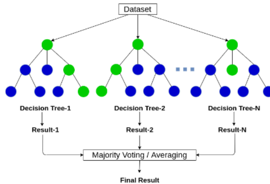
Fig. 3.7 Random Forest Prediction Model
