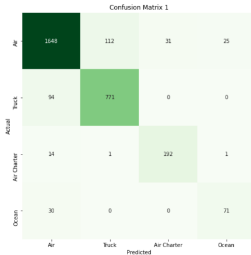
Fig. 4.1 Confusion Matrix of predicted shipment mode
