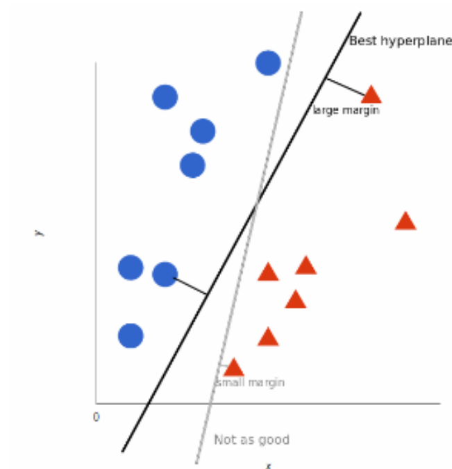
Fig. 3.6 Hyperplane formed using SVM
