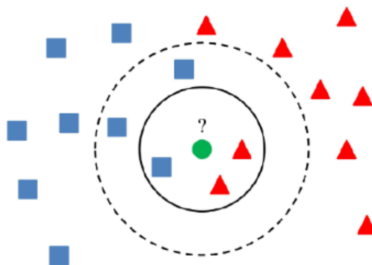
Fig. 3.3 K-Nearest Neighbour
